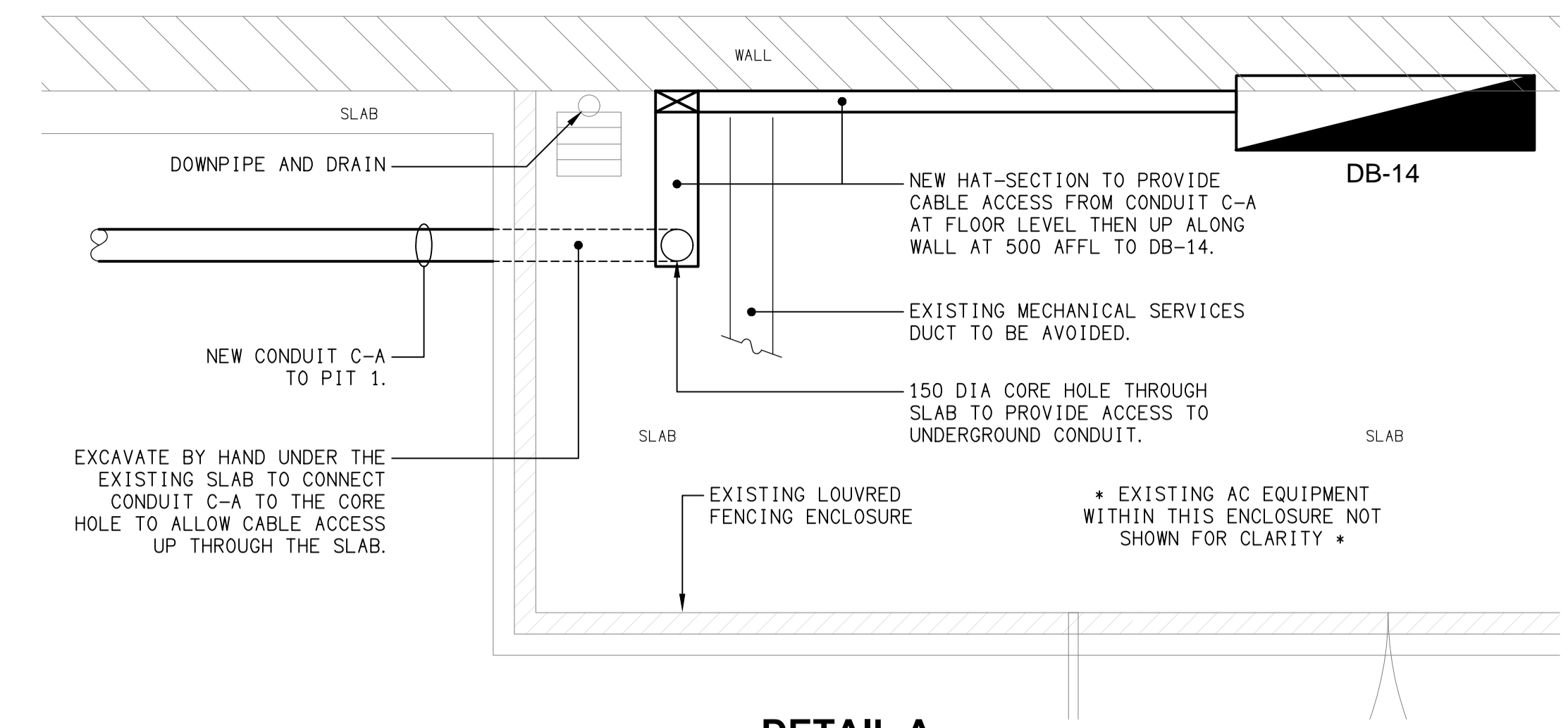
DETAIL A DB-14 CABLE ACCESS PLAN VIEW NOT TO SCALE
